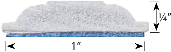
SDL Bar Profile
